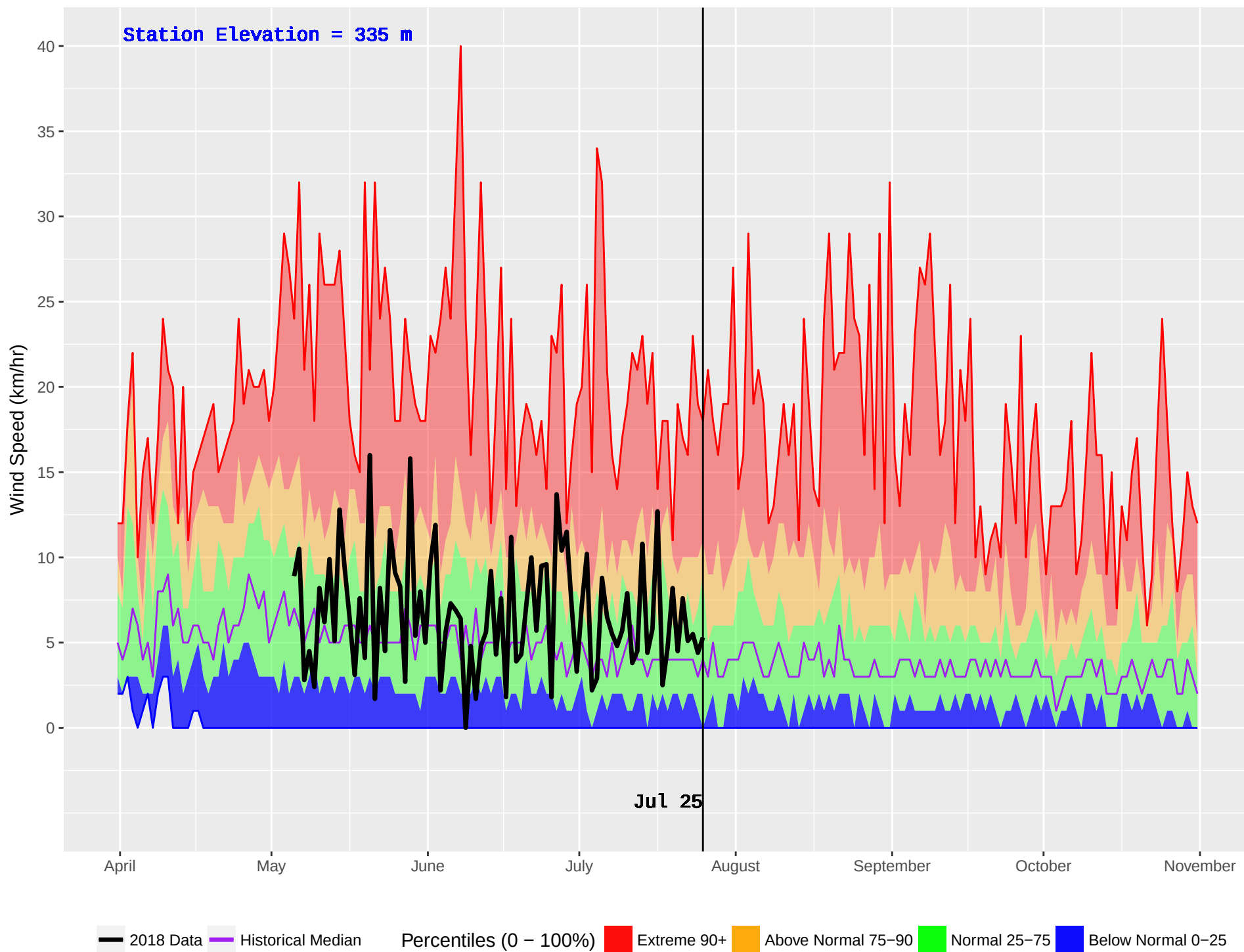
KISPIOX HUB (428) : Historical (1970–2016) and Current (2018) Noon Wind Speed
