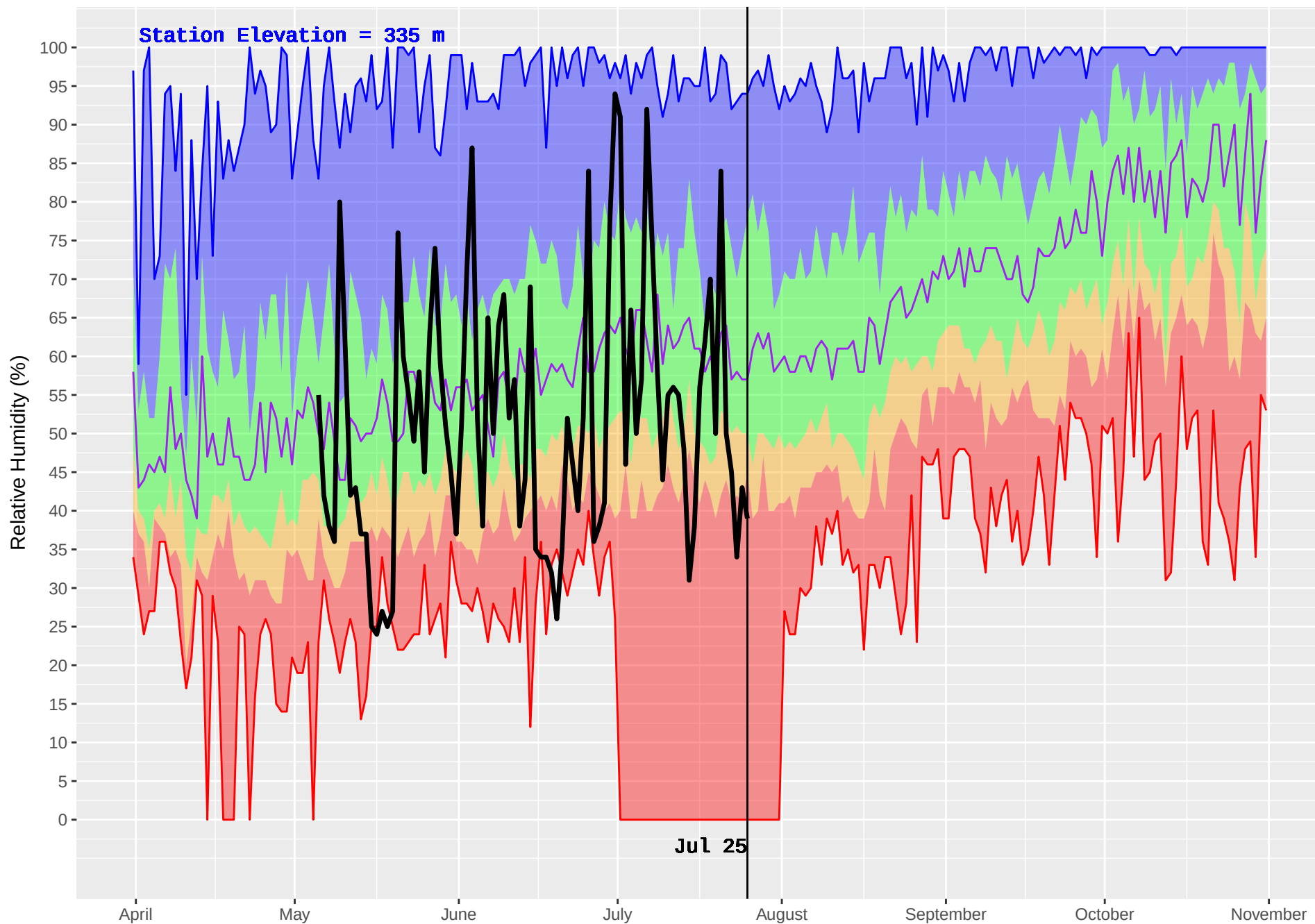
KISPIOX HUB (428) : Historical (1970–2016) and Current (2018) Noon Relative Humidity
