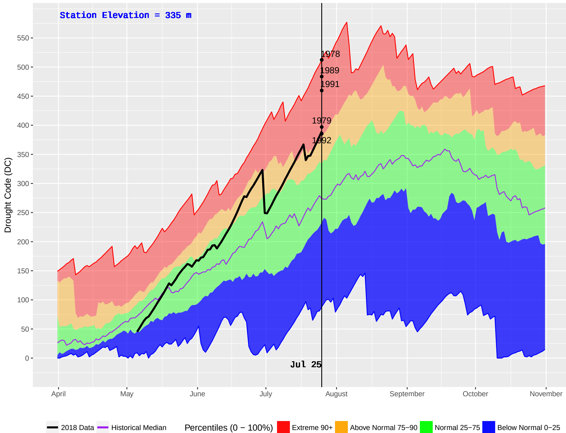
KISPIOX HUB (428) : Historical (1970–2016) and Current (2018) Noon Drought Code (DC)
