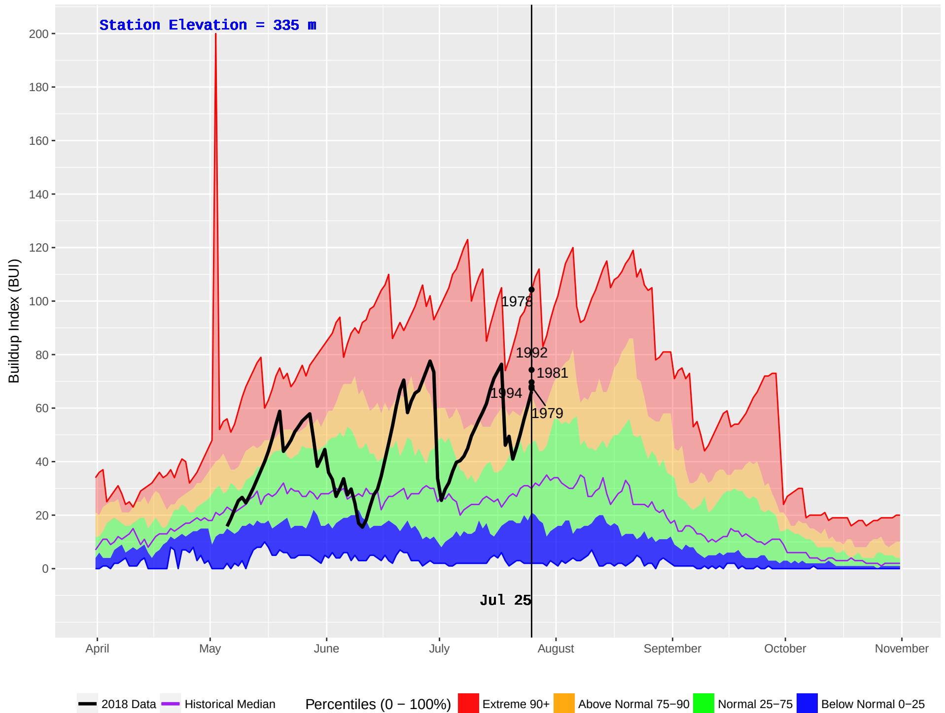
KISPIOX HUB (428) : Historical (1970–2016) and Current (2018) Noon Buildup Index (BUI)
