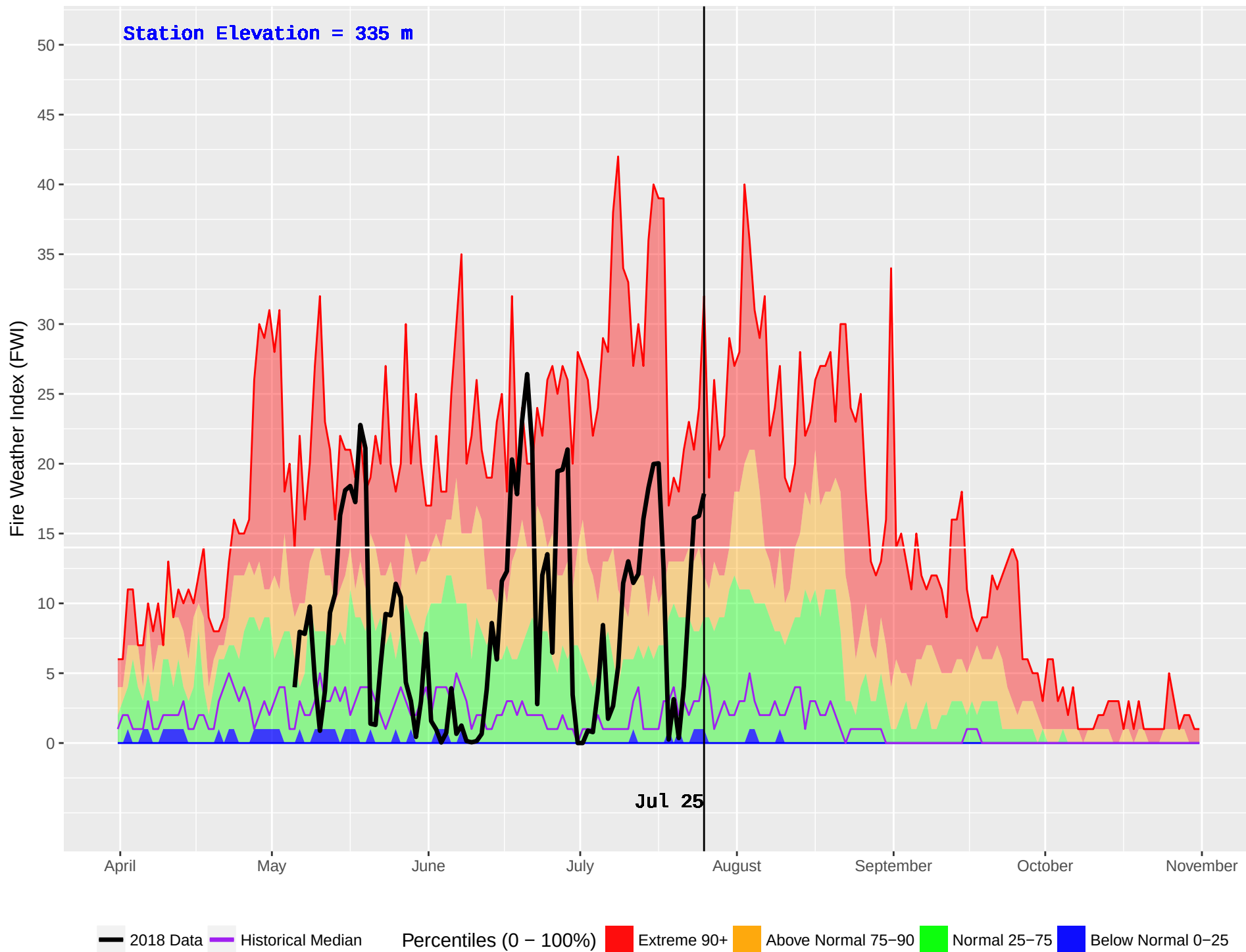
KISPIOX HUB (428) : Historical (1970–2016) and Current (2018) Noon Fire Weather Index (FWI)
